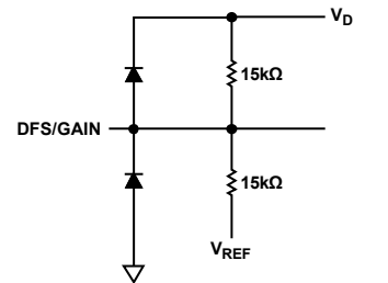
Figure 13. DFS/Gain Input
